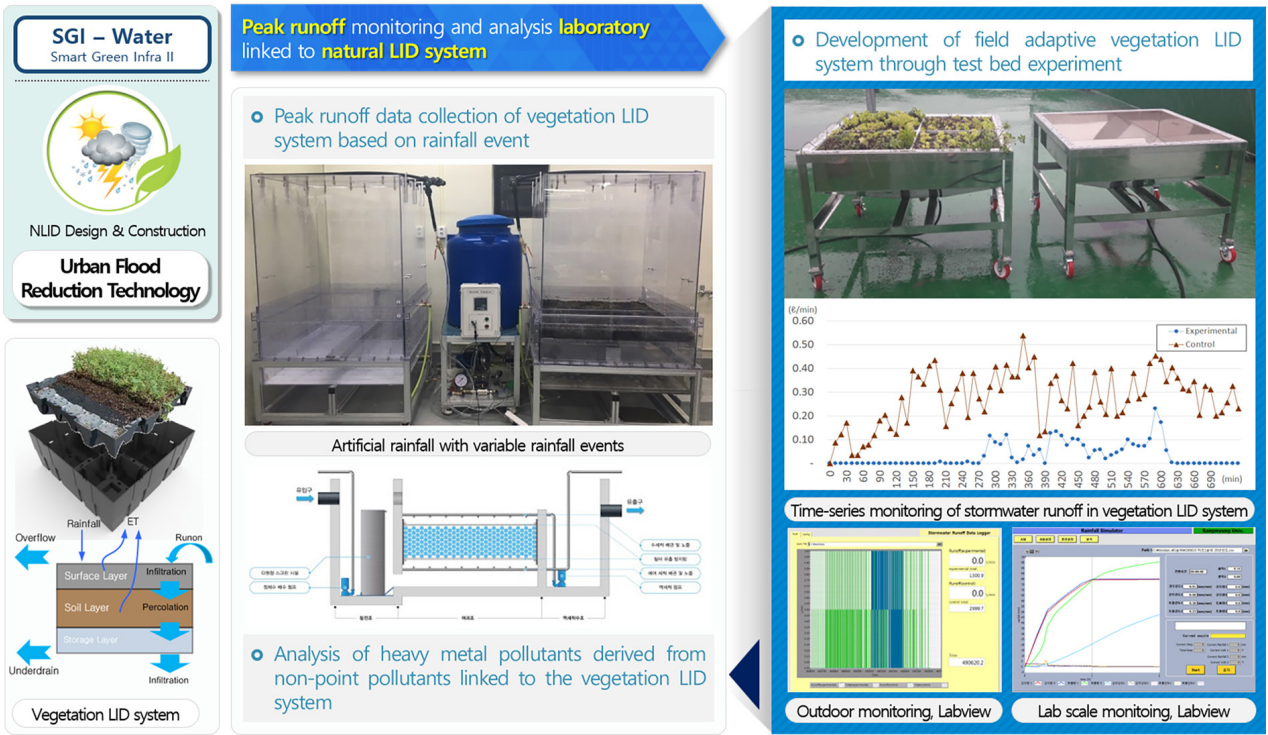
Figure 4: Smart Green Infrastructure-Water
