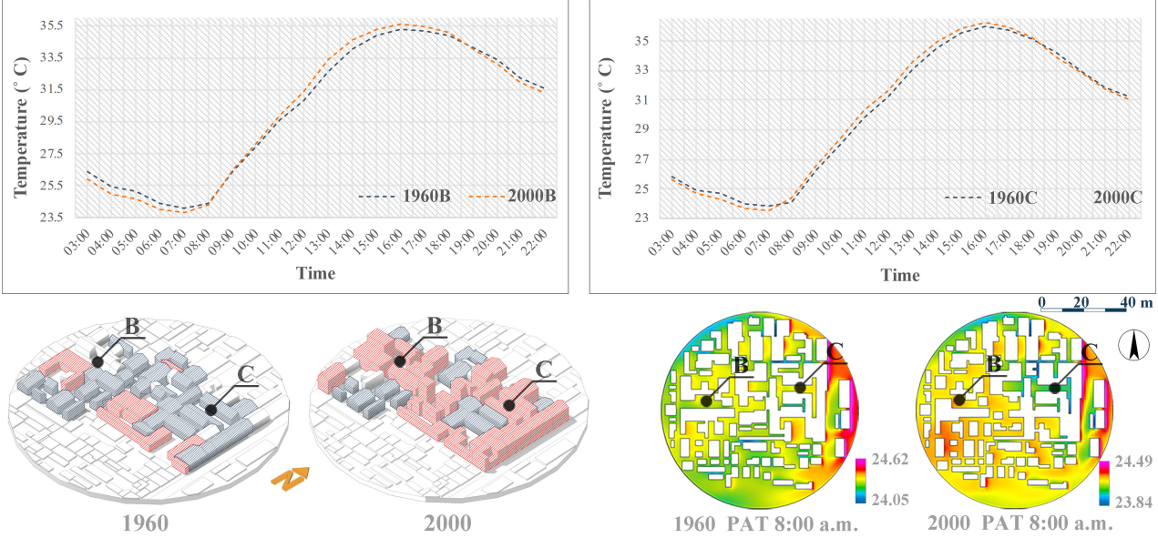
Figure 6. Comparison diagram of thermal environment of courtyards with different surrounding building heights
